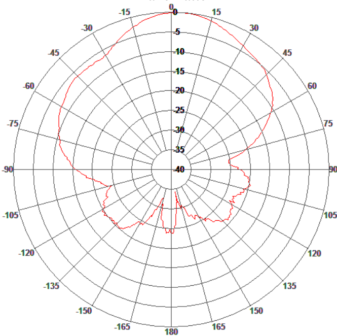
E-Plane Pattern
