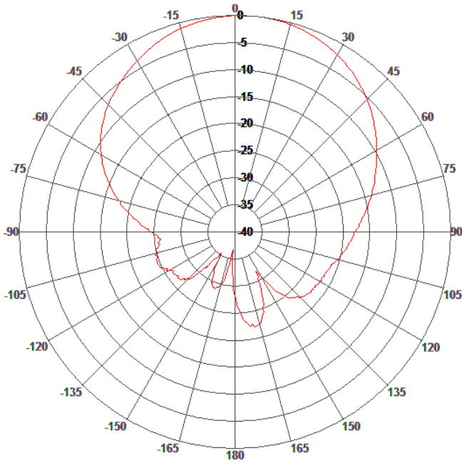
E-Plane Patterns
