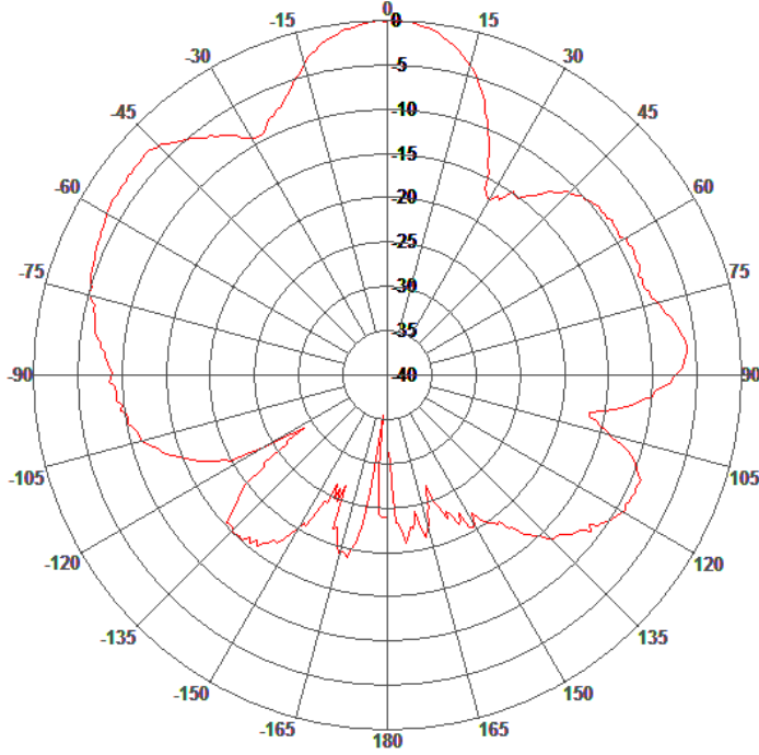
E-Plane Patterns
