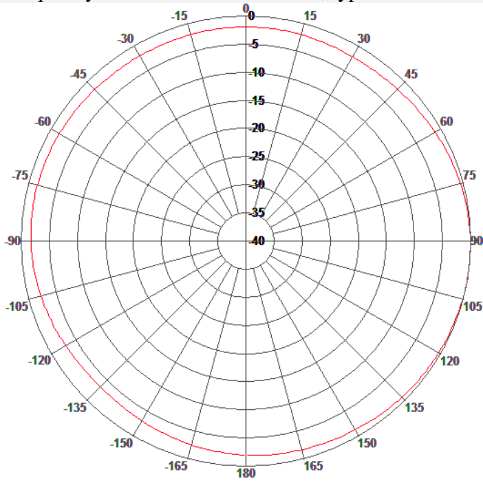
Frequency 3400 MHz
