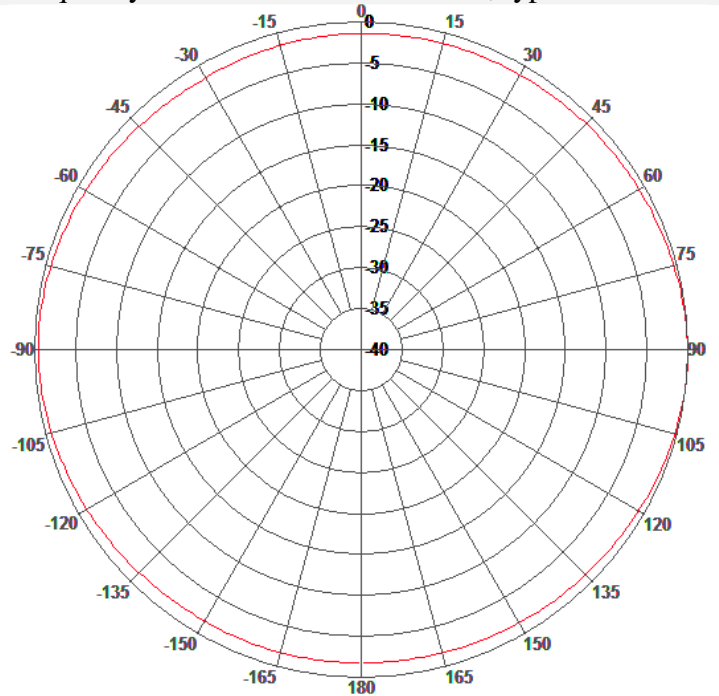
Frequency 1710 MHz
