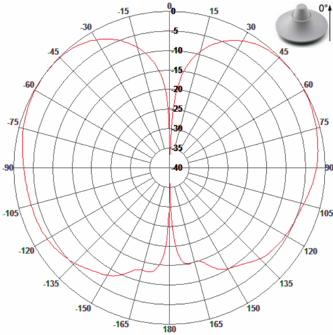
E-Plane Patterns
