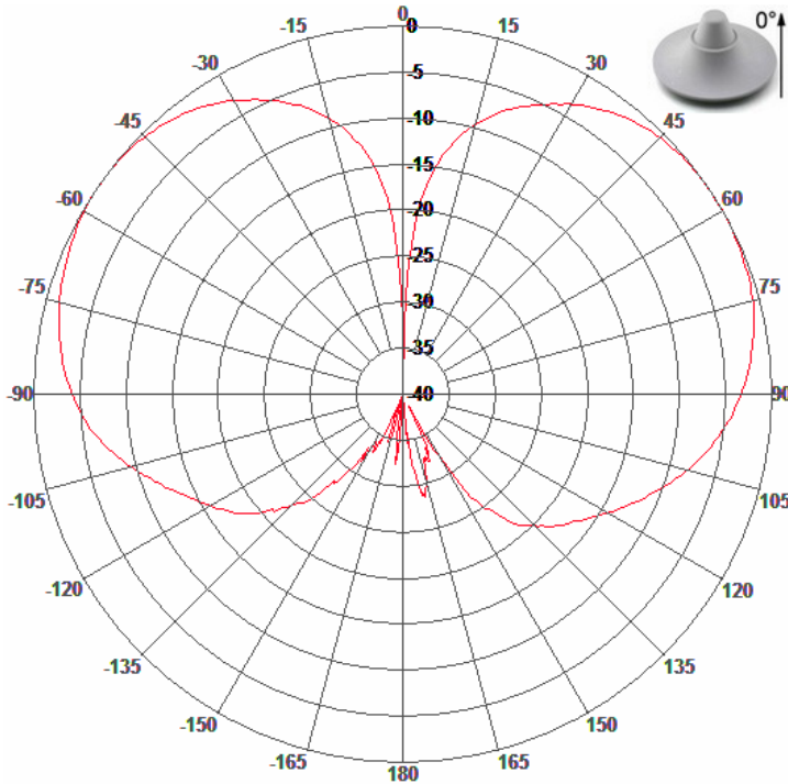
E-Plane Pattern
