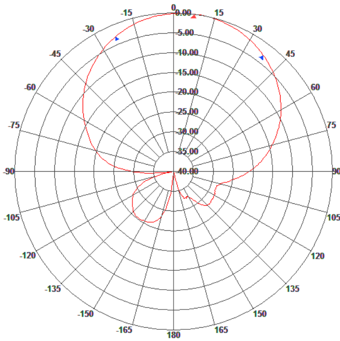
E-Plane Pattern
