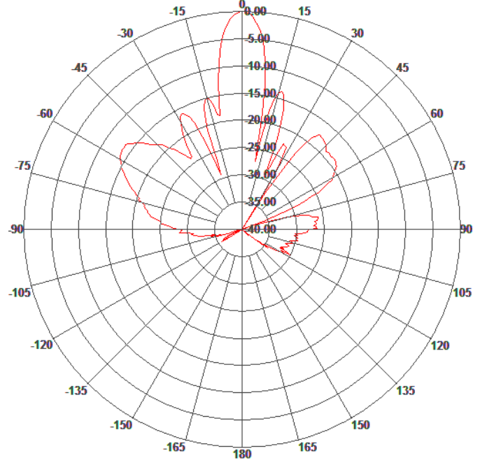
Elevation Pattern
