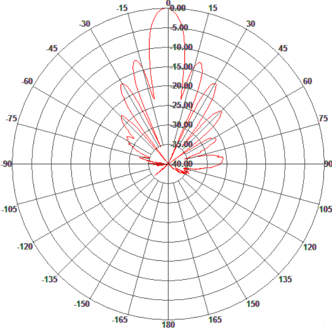
Azimuth Pattern
