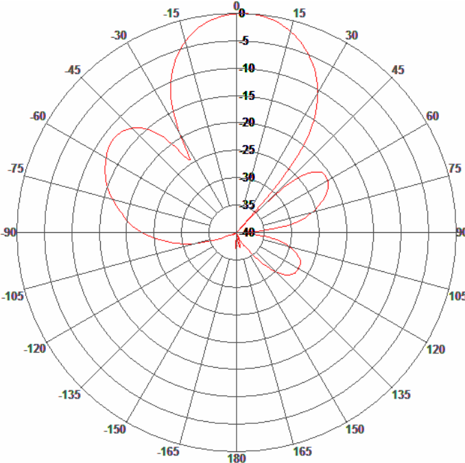
E-Plane Pattern
