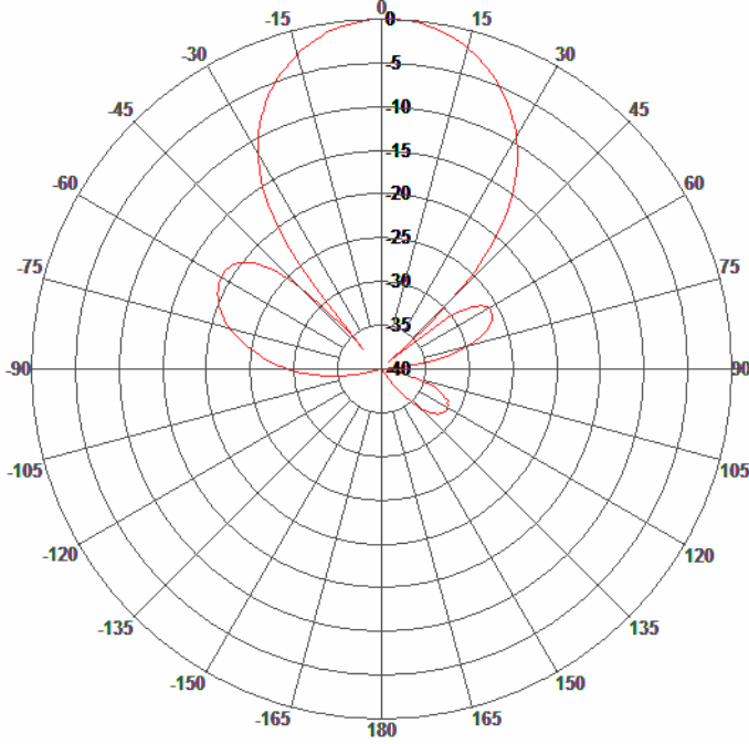
E-Plane Pattern
