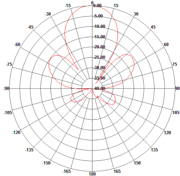
Azimuth Pattern
