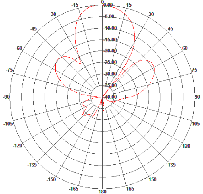
Elevation Pattern
