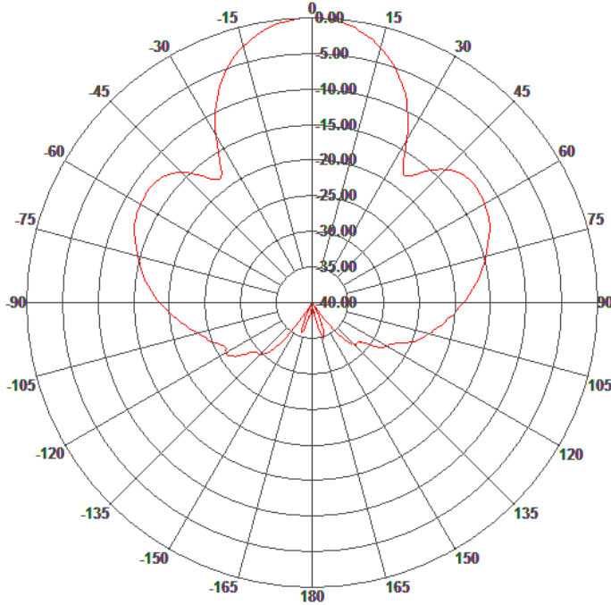
Azimuth Pattern
