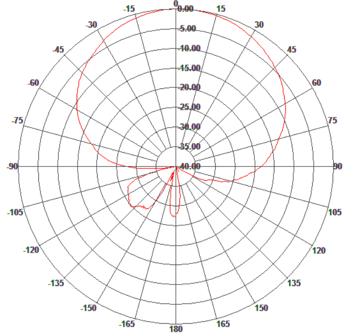
Elevation Pattern
