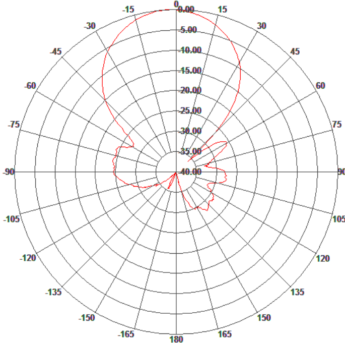
Azimuth Pattern
