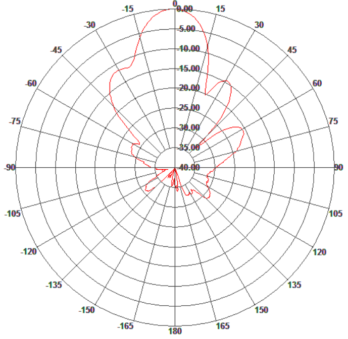
Elevation Pattern
