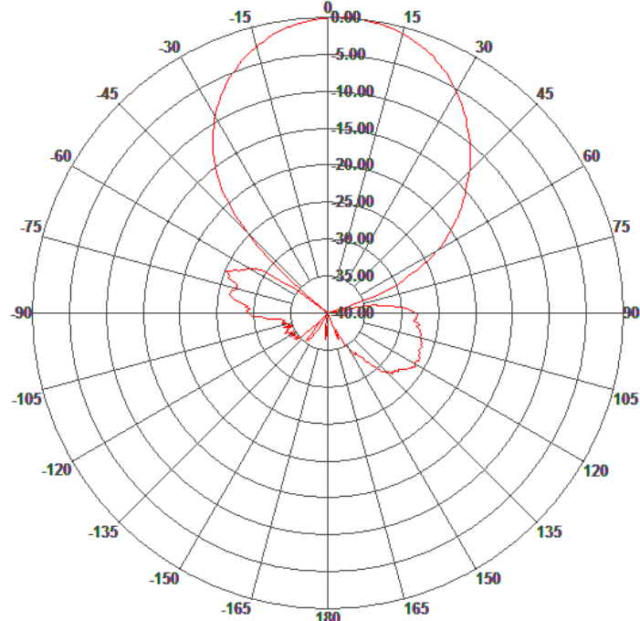
Elevation Pattern
