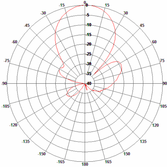
E-Plane Pattern
