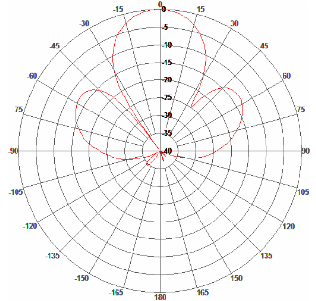
E-Plane Pattern
