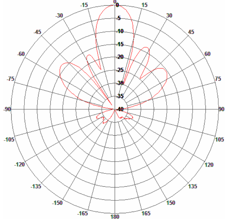
Elevation Pattern
