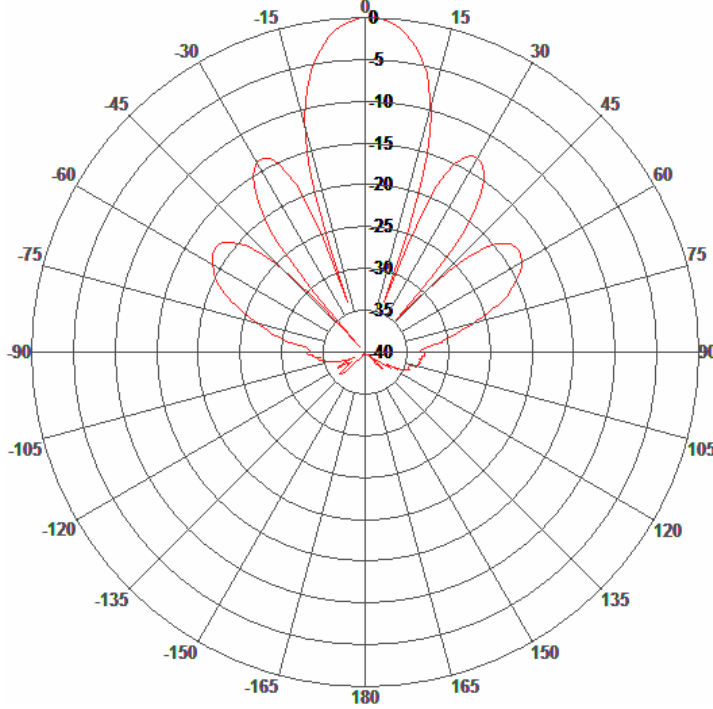
Azimuth Pattern
