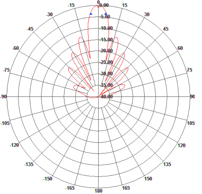
Elevation Pattern
