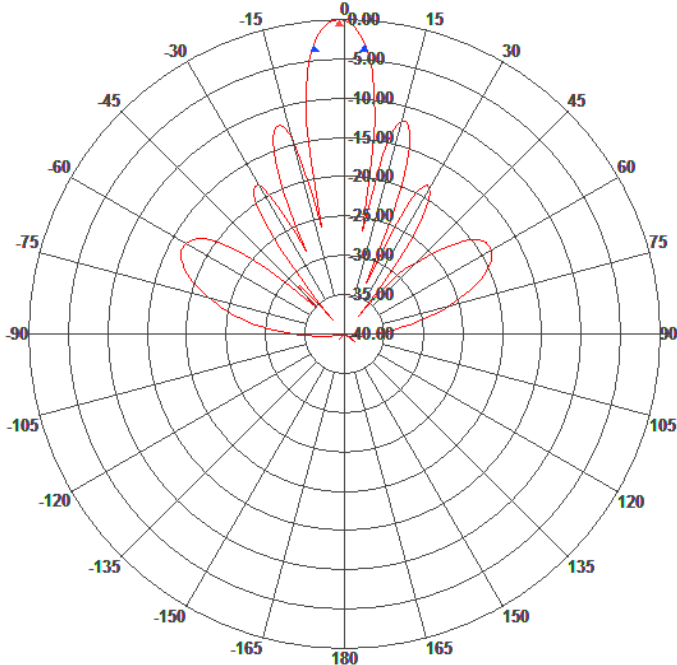
Azimuth Pattern
