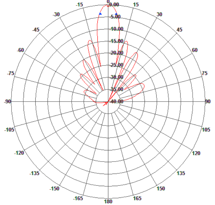
Elevation Pattern
