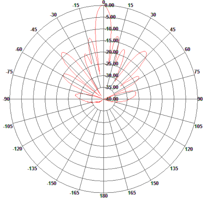
Elevation Pattern
