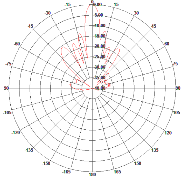
Azimuth Pattern
