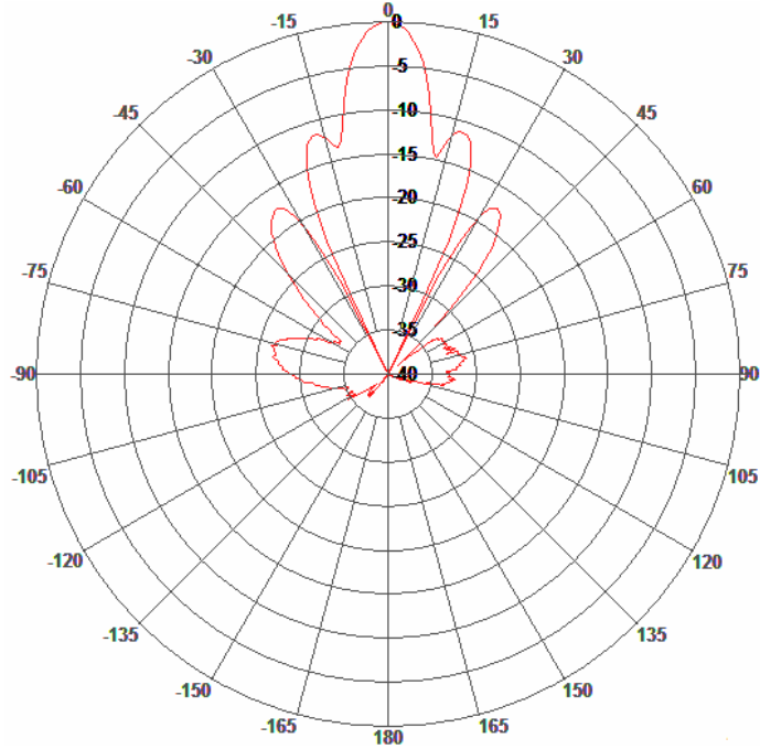
E-Plane Pattern
