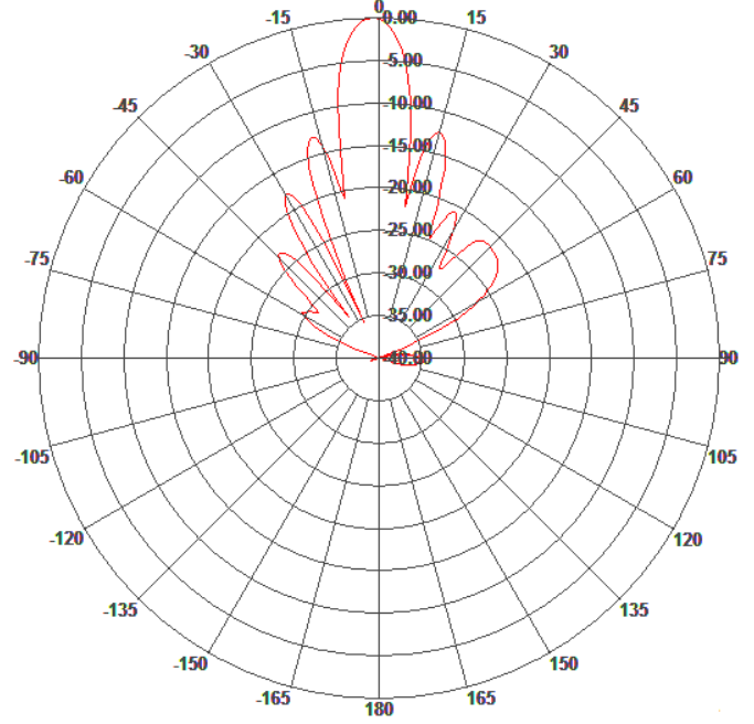
Elevation Pattern
