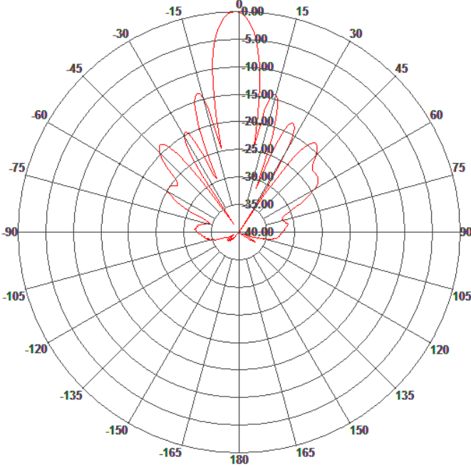
Azimuth Pattern
