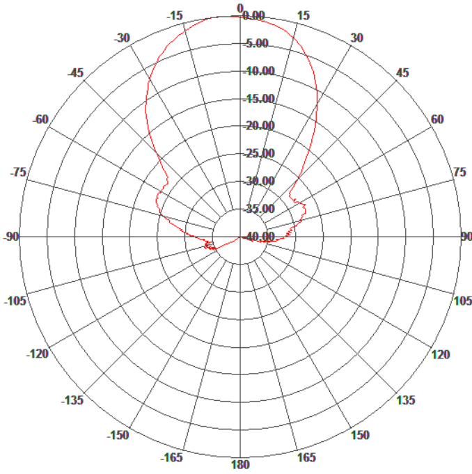
Azimuth Pattern
