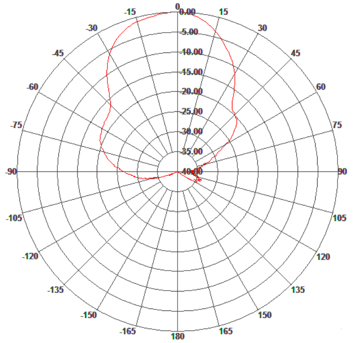
Elevation Pattern
