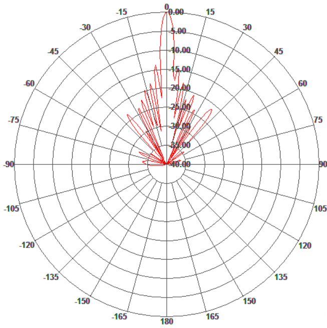
E-Plane Pattern
