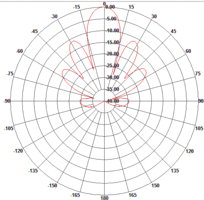
Elevation Pattern
