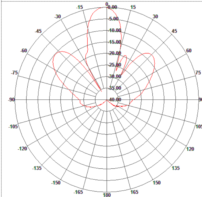
Azimuth Pattern
