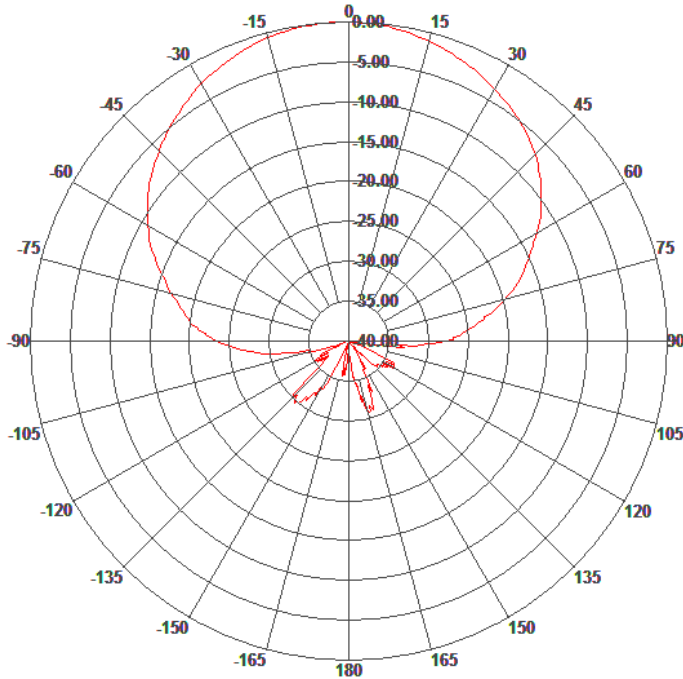
E-Plane Patterns
