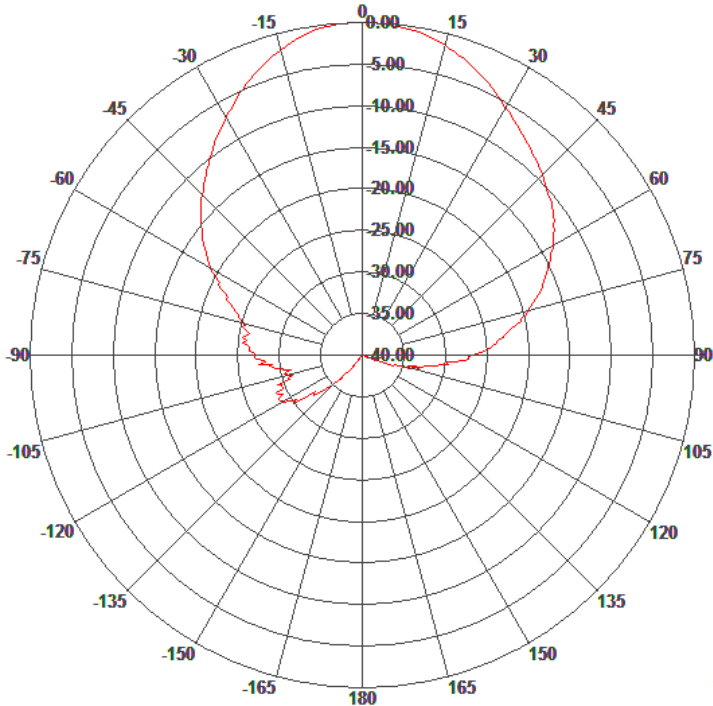
E-Plane Pattern
