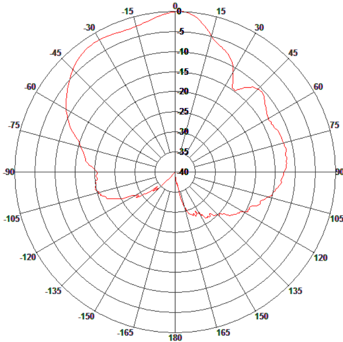
E-Plane Pattern
