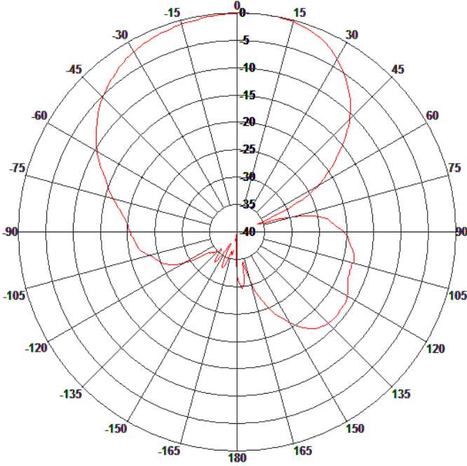
E-Plane Patterns
