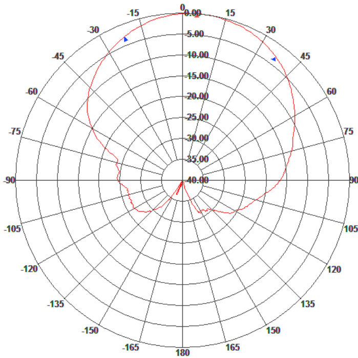
E-Plane Patterns
