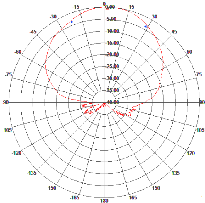
E-Plane Pattern
