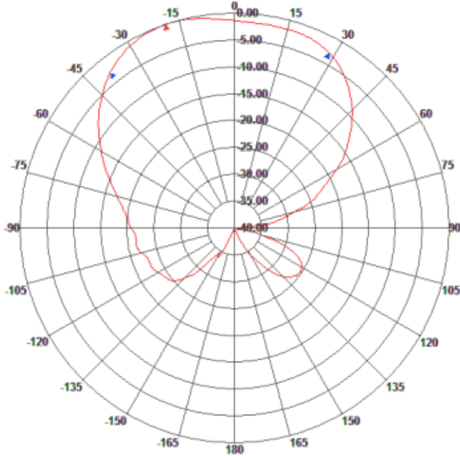
Azimuth Patterns
