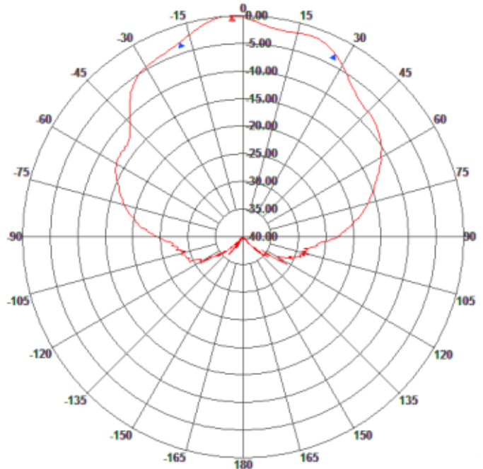
Elevation Patterns
