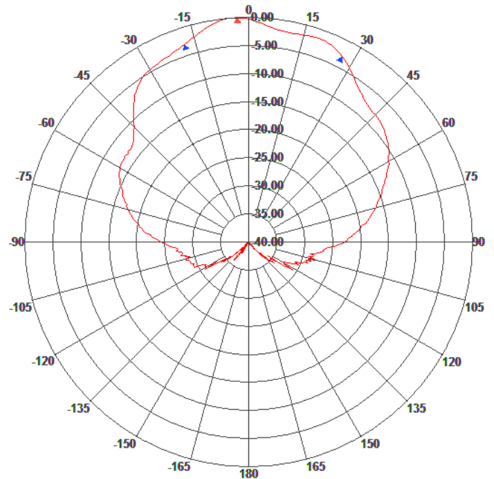
Elevation Patterns
