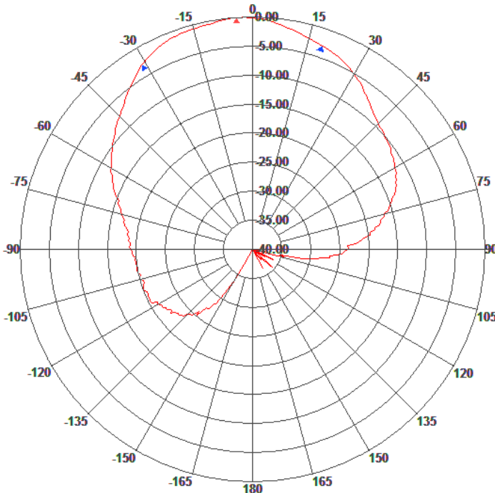
Azimuth Patterns
