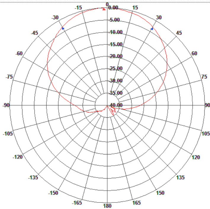
Azimuth Pattern
