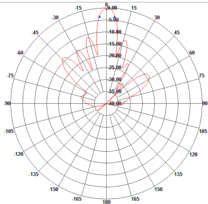
Elevation Pattern
