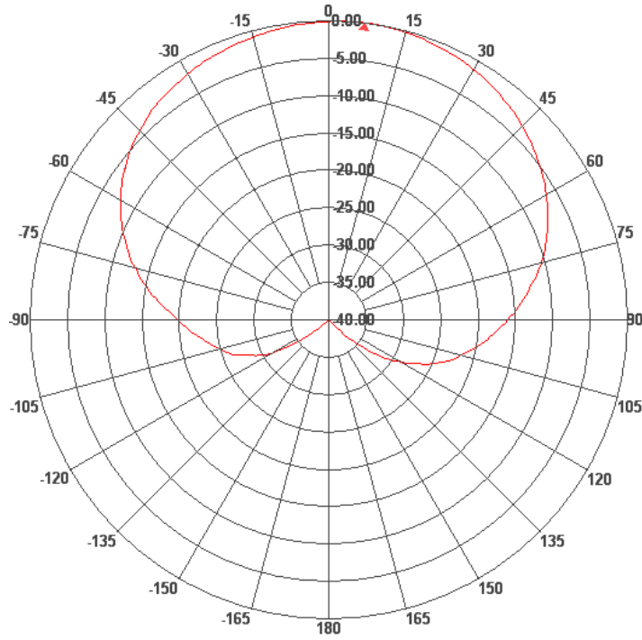
Azimuth Pattern
