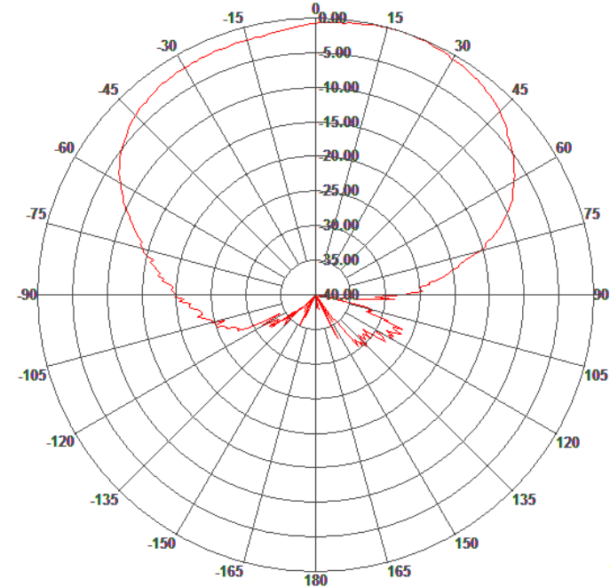
Azimuth Pattern
