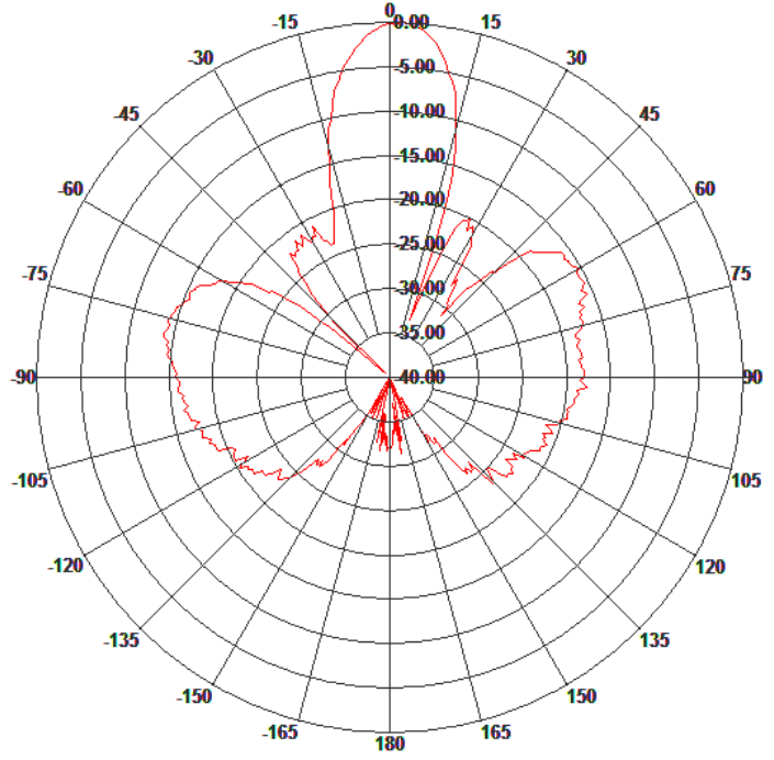
Elevation Pattern
