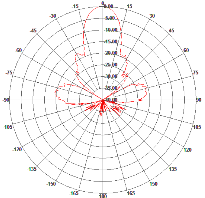
Elevation Pattern
