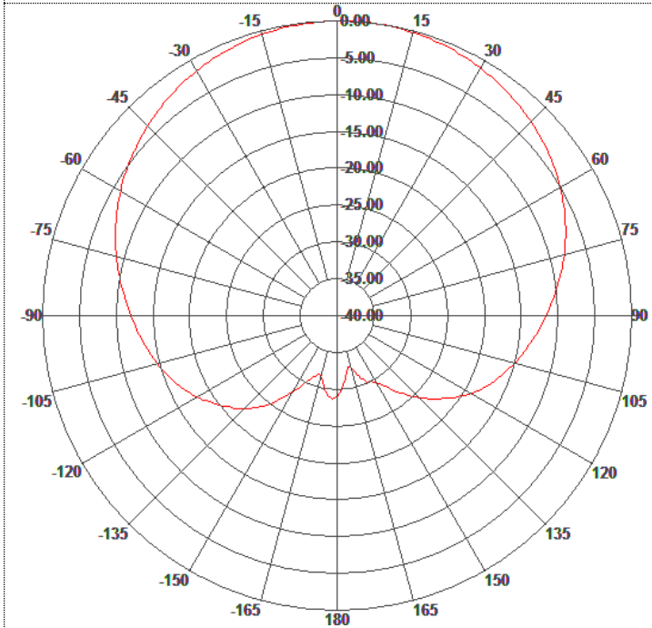
Azimuth Pattern
