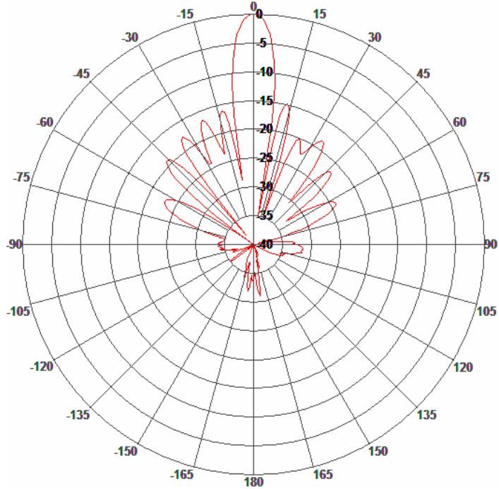
E-Plane Pattern
