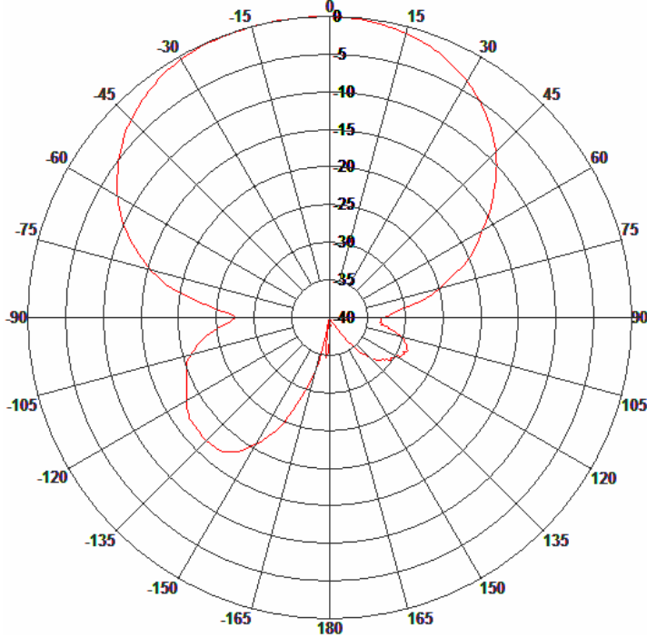
E-Plane Patterns
