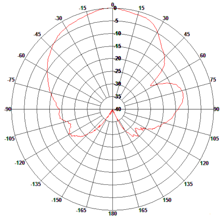
E-Plane Pattern
