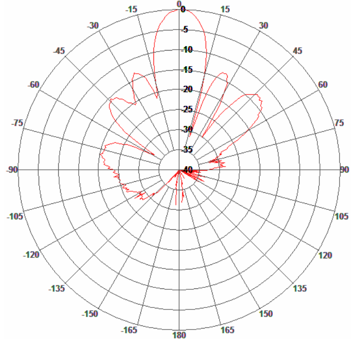
Elevation Pattern
