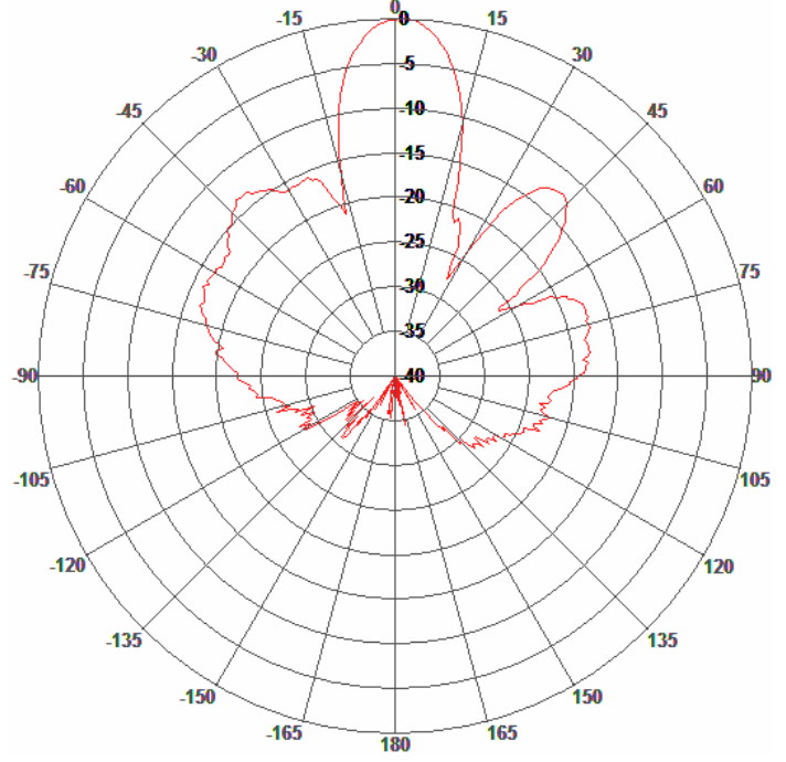
Elevation Pattern
