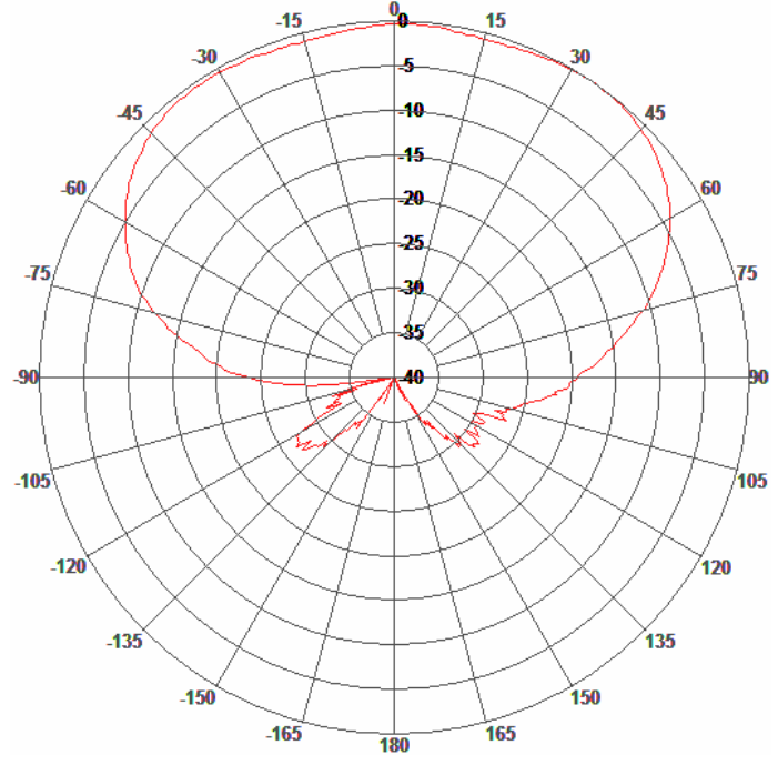
Azimuth Pattern
