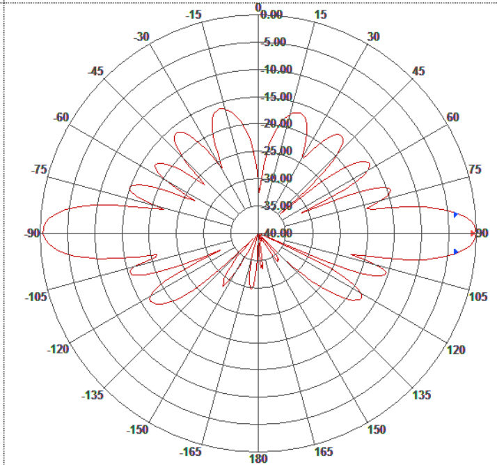
Elevation Pattern
