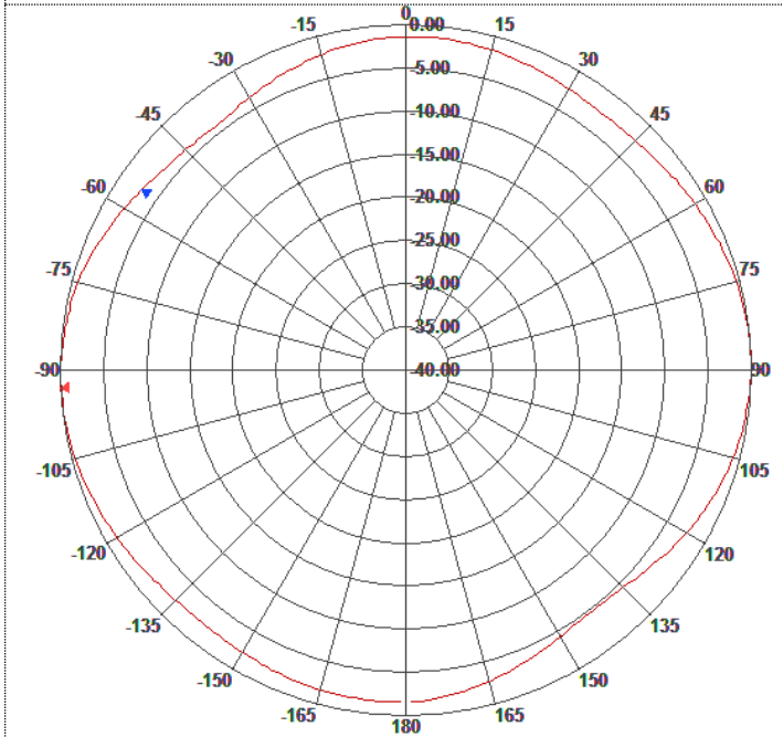
Azimuth Pattern
