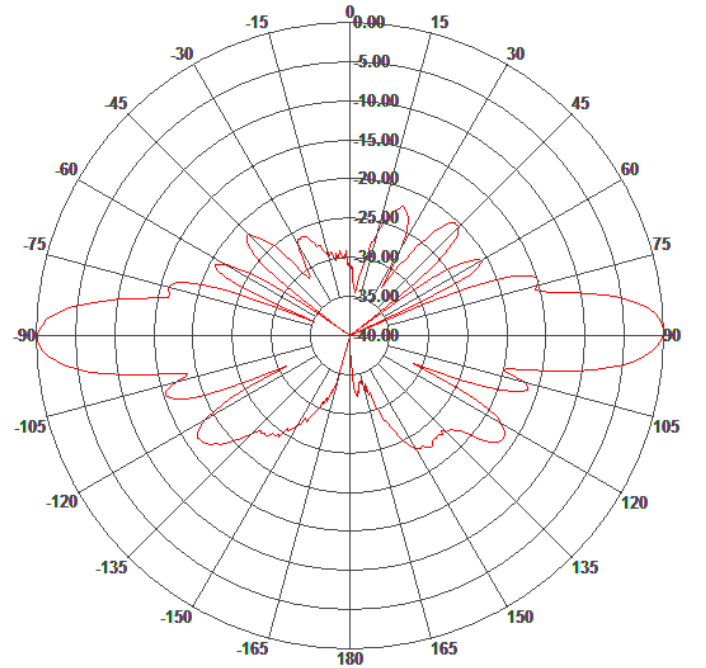
Elevation Pattern
