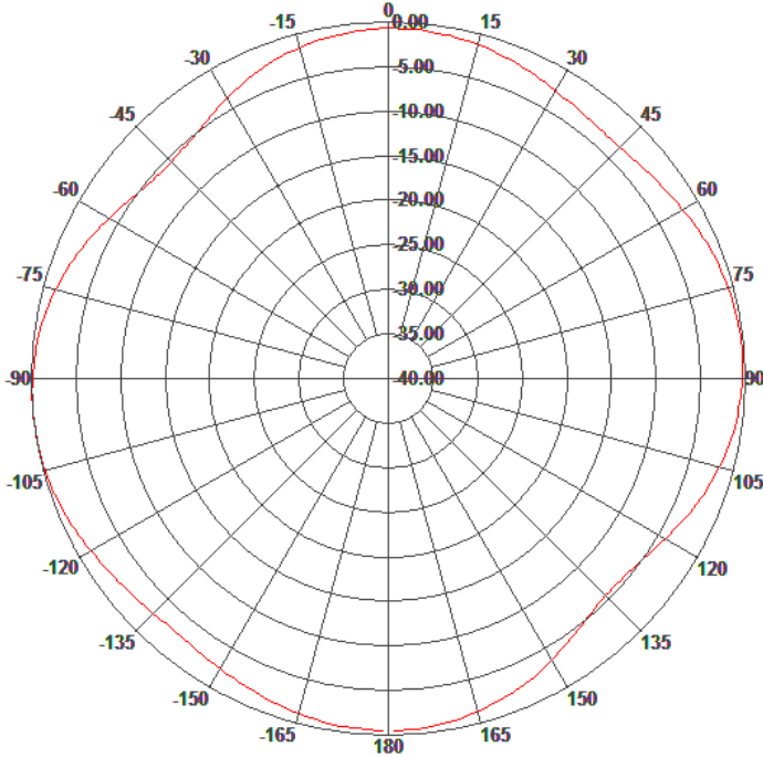
Azimuth Pattern
