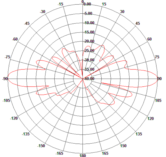
Elevation Pattern
