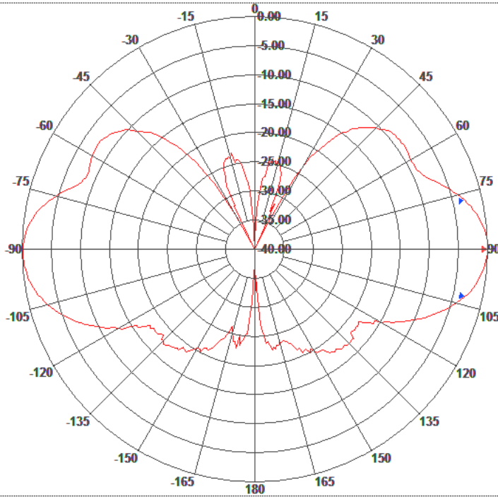
Elevation Pattern
