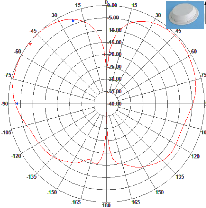
E-Plane Pattern
