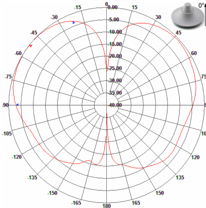
E-Plane Pattern
