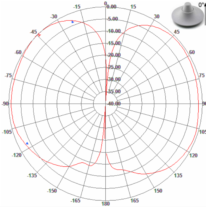
E-Plane Patterns
