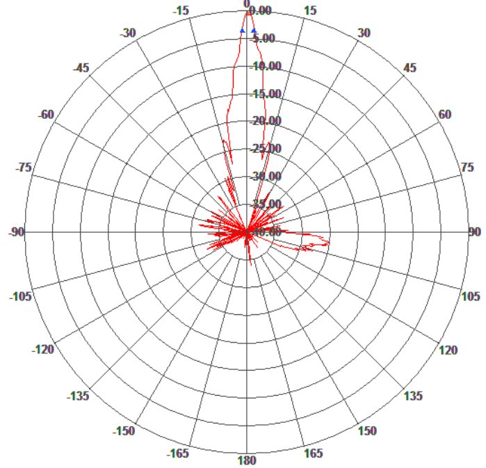
Azimuth Pattern
