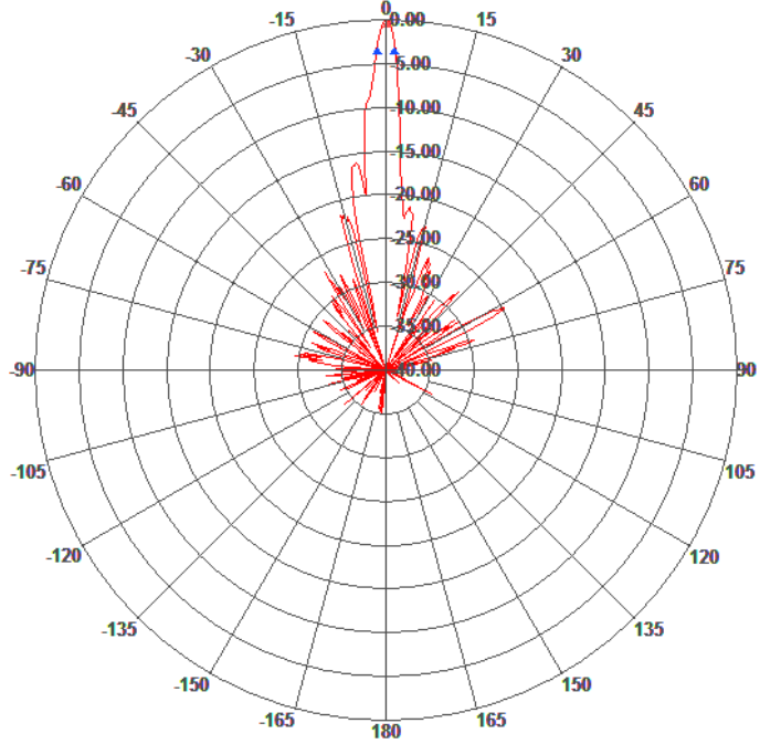
Elevation Pattern
