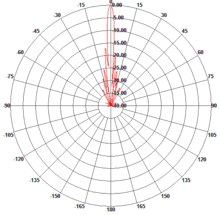
Elevation Pattern
