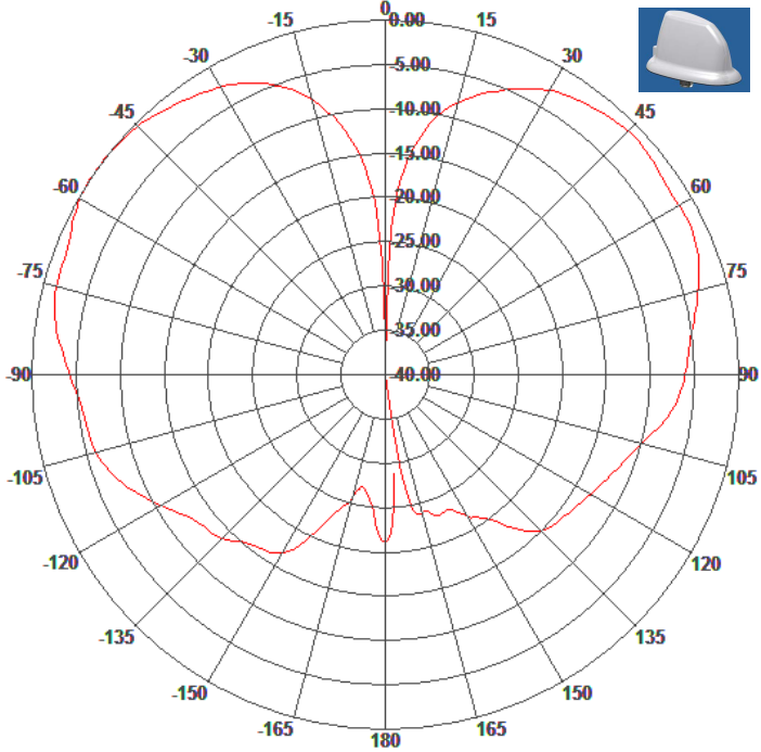
E-Plane Patterns
