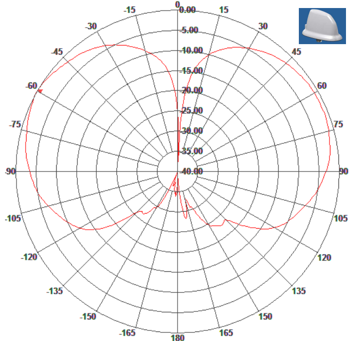
E-Plane Pattern
